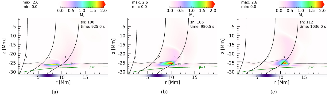
Fig. 2: Snapshots of the parallel Mach number M_s = |\hat{v}_{||}|/c_s in the wave-driven simulation at times corresponding to (a) t = 925 s, (b) t = 981 s and (c) t = 1036 s. An animated version of this figure is available online in addition to an animated version of the Mach values in the un-driven simulation.
