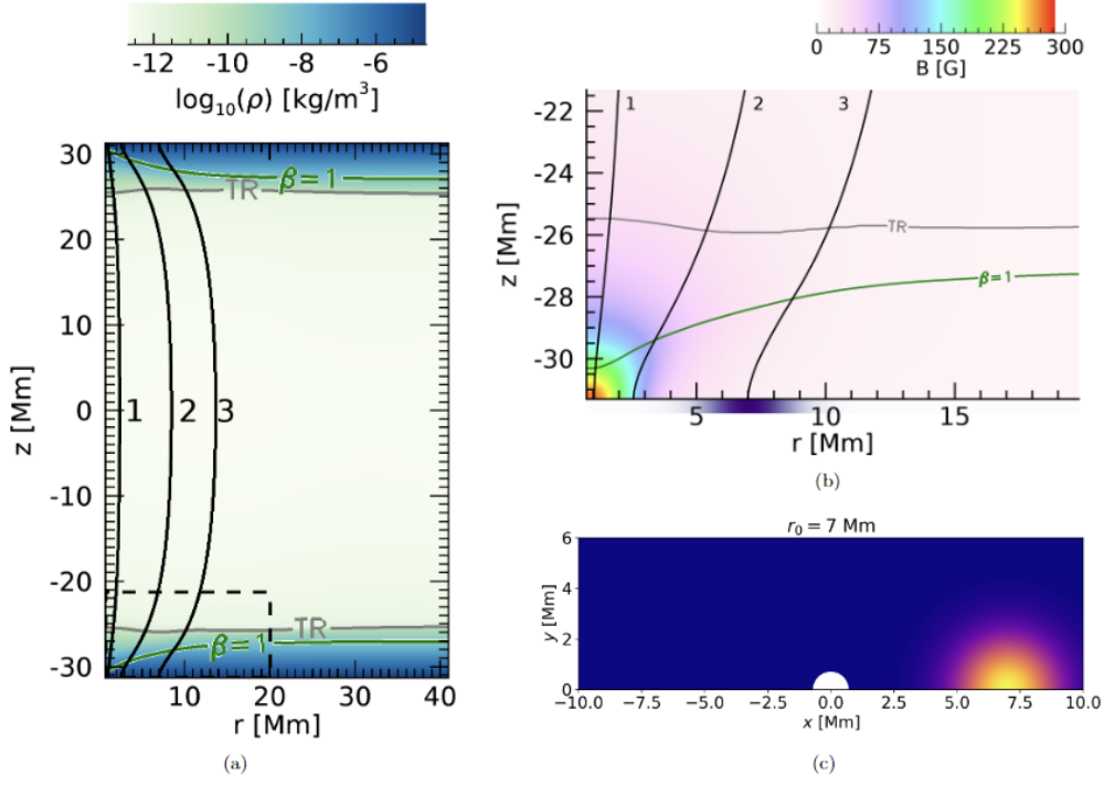
Fig. 1: (a) The initial background density (plotted on a log scale) in the full simulation domain at an azimuthal slice \varphi = 0 . The positions of field lines 1, 2 and 3 indicated for discussion in the text. Contours for the plasma- \beta = 1 layer and transition region are shown by the green and grey lines, respectively. Panel (b) shows the initial magnetic field strength and topology outlined by the black dashed box in panel (a). The same configuration is found for all azimuthal angles due to the symmetry of the background equilibrium around the central axis. The location and strength of the (asymmetric) wave driver is highlighted by the purple bar on the horizontal axis. (c) The location of the wave driver employed with r_0 = 7 Mm (displayed on a Cartesian grid). The strength of the driver is shown in arbitrary units.
