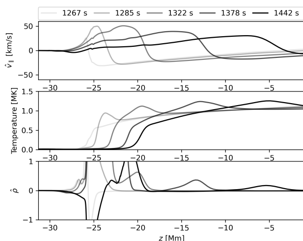
Fig. 4: The time evolution of the velocity perturbation along field line 3 ( \hat{v}_{\parallel} ) in the simulation with a photospheric wave driver, the temperature along field line 3 and the density perturbation ( \hat{\rho} ) along field line 3 calculated using Equation (1). An animated version of this figure is available online.
