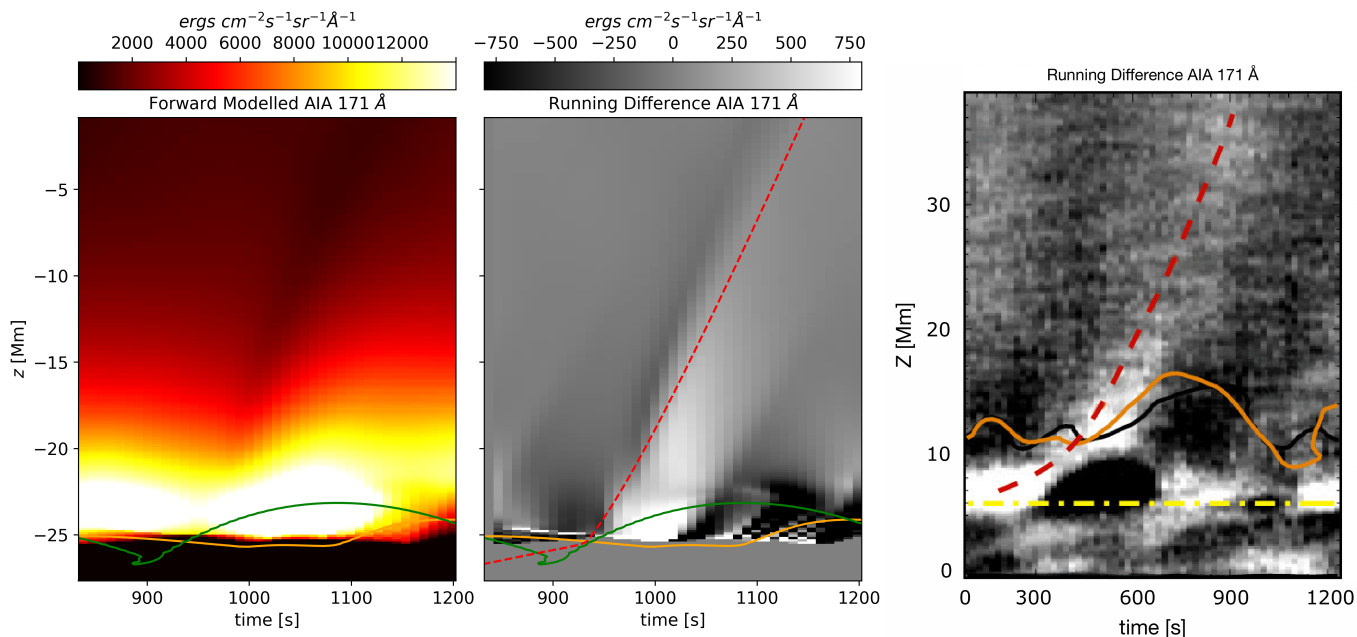
Fig. 9: Left: Synthetic AIA 171 Å time-distance diagram produced using an artificial slit at r = 12.5 Mm. The green contour shows the location of the transition region ( T=40,000 K) in the simulation with a photospheric wave driver measured along field line 3, whereas the orange contour displays the same temperature contour using a vertical slit at r = 12.5 Mm. Middle: Running difference AIA 171 Å highlighting the nature of the PD in the simulation. The red dashed line highlights the trajectory of the sound speed in the simulation domain. Right: Observation from Samanta et al. (2015) of AIA 171 Å running difference where the orange and black contours outline the height of the transition region using observations from IRIS 2796 Å and IRIS 1400 Å channels. The red dashed line indicates the determined sound speed from the observations whereas the dashed-dot yellow line outlines the solar limb as observed in AIA instruments.
