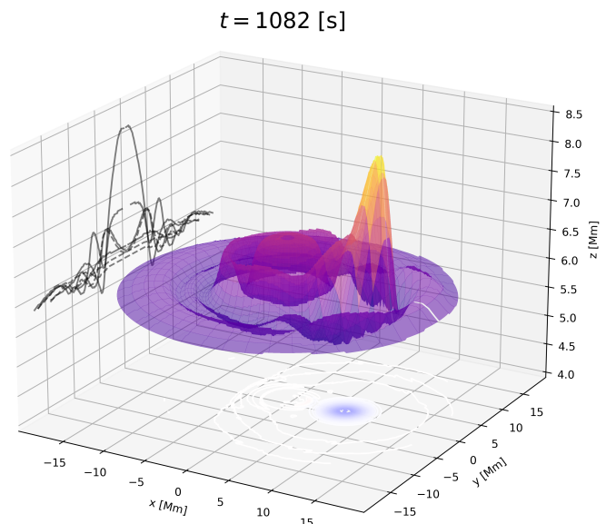
Fig. 5: A 3D representation of the height (above the bottom boundary of the simulation) of the transition region, calculated as a temperature contour of 40,000 K at a specific snapshot in time of t = 1082 s. The strength of the v_z perturbation is shown on the bottom boundary plane and the shadow contour of the transition region height is projected against the y - z plane to highlight the surface waves formed at the transition region resulting from previous spicule launches.
