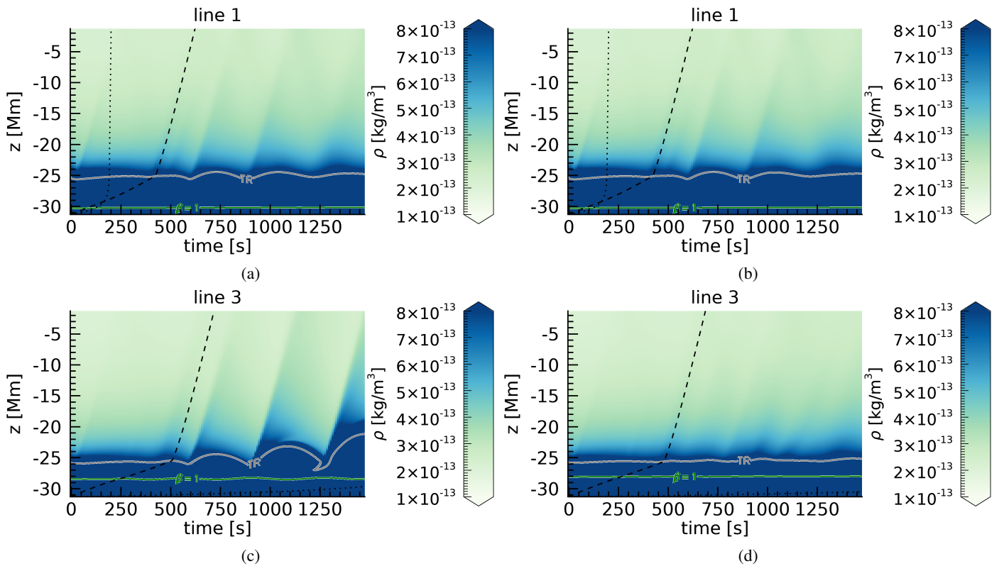
Fig. 6: Time-distance plots of the density in the simulation where an acoustic gravity wave driver is positioned at r = 7 Mm, for the three field lines indicated in Figure 1 at an azimuthal slice \varphi = 0 . Locations of the transition region and plasma- \beta = 1 layer are indicated by the grey and green contours respectively. We also display the local sound speed (dashed line) and local Alfvén speed (dotted line) in each plot. The colour bar is saturated at the upper limit to aid visualisation.
