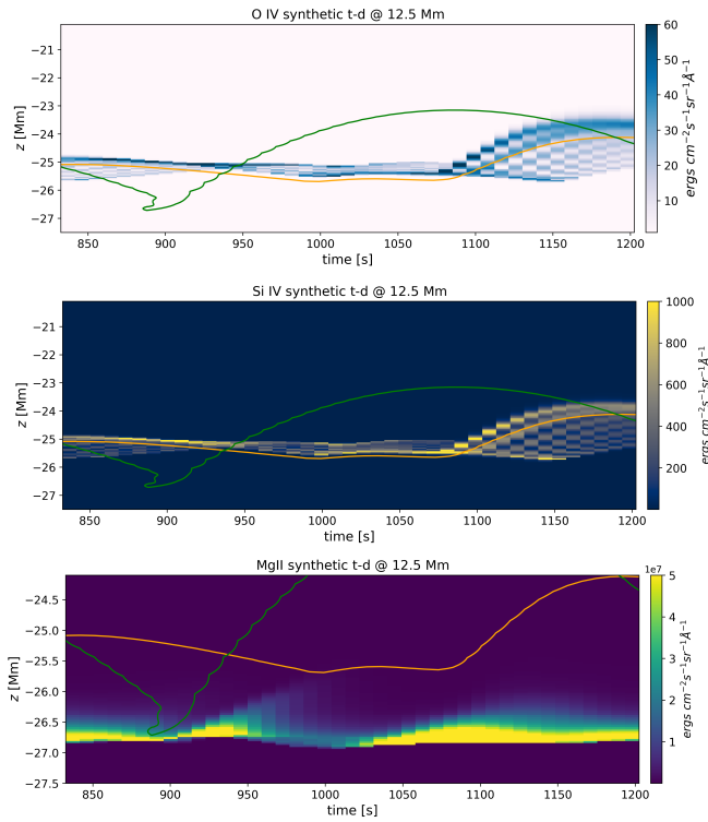
Fig. 11: Time-distance plots of optically thin transition region lines O IV (top), Si IV (middle) and Mg II (bottom) from the simulation with a photospheric wave driver along a vertical slit at r = 12.5 Mm. The height axis is zoomed in on the transition region. The green and orange lines have the same representation as outlined in Figure 9.
