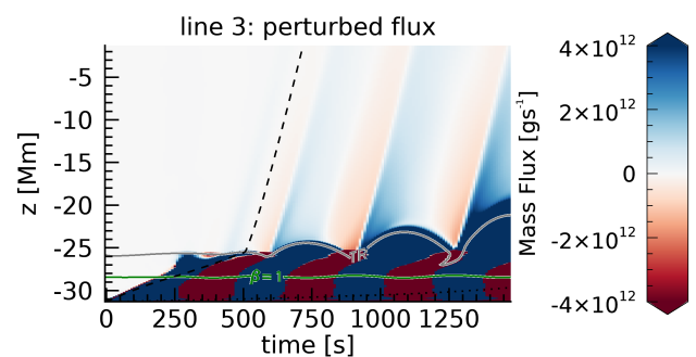
Fig. 8: Time-distance plot of the perturbed mass flux associated with PDs from the simulation with a wave driver along field line 3 at an azimuthal slice \varphi = 0 calculated using Equation (3) with the density perturbation \hat{\rho} determined from the simulation with a wave driver minus the simulation without a wave driver.
